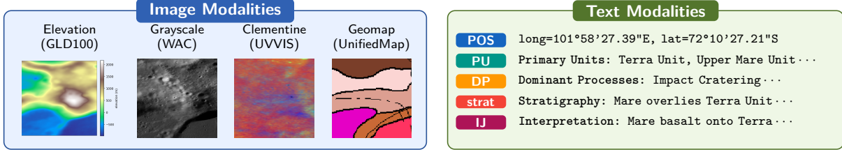
Figure 2: Overview of the input modalities. All raster products are co-registered at 100 m/pixel. The text modalities are derived from per-tile coordinates and from weakly supervised captions.
