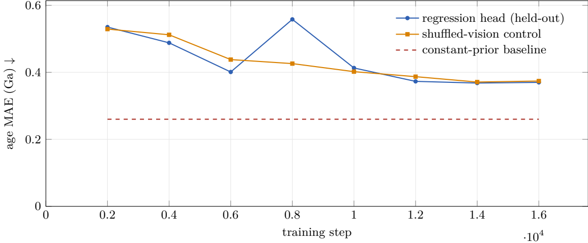
Figure 9: Held-out age MAE of the in-loop supervised age head, a regression head trained jointly on the mean-pooled resampler output (mare-gated Huber loss), evaluated per training snapshot ( n = 40 ). The constant-prior baseline is recomputed on this evaluation’s own set of n = 40 dated snapshot tile sets (Sec. 5.3) and is therefore lower than the constants of Tables 3 and 7, which live on different tile sets. The head never beats this baseline, and the shuffled-vision control tracks it closely. Together with the frozen-resampler probe (Table 8), the localization is that the representation the head reads provably carries the signal, and the joint training fails to extract it (Sec. 7.6).
