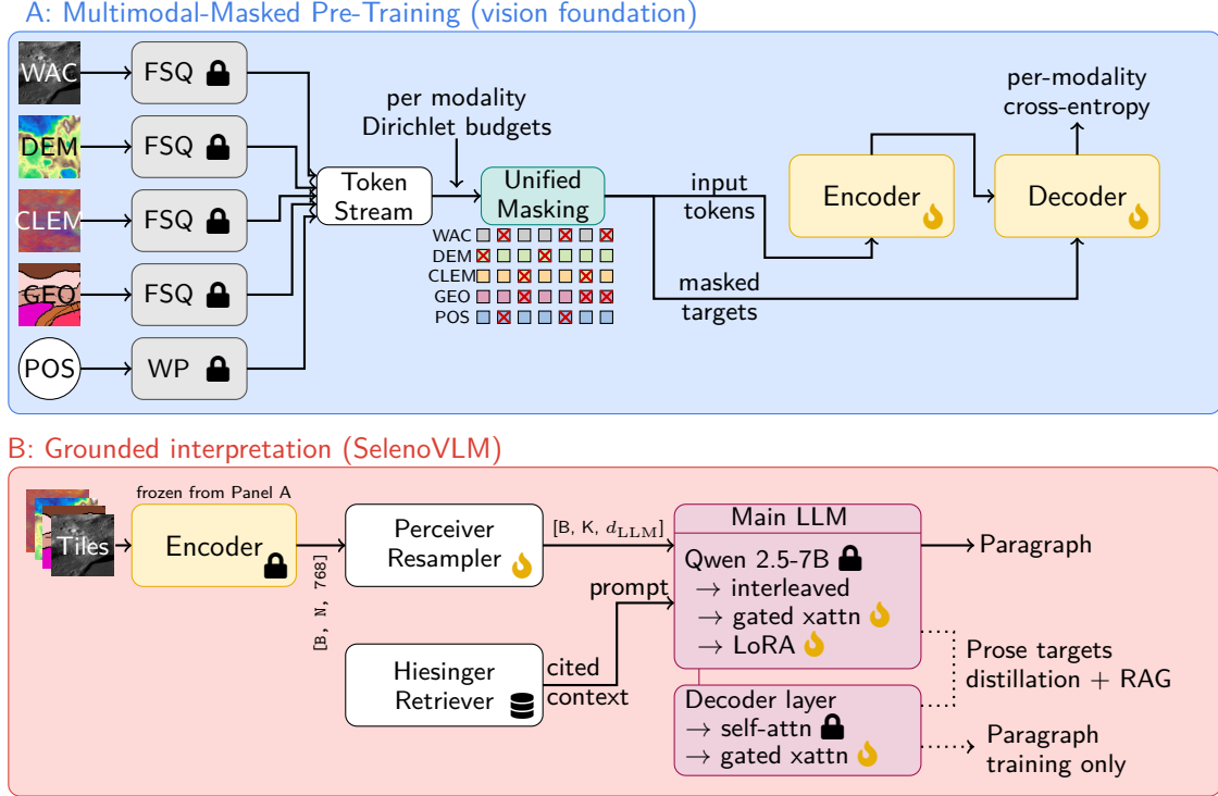
Figure 3: Overview of the proposed two-stage methodology. (A) Multimodal-masked pre-training. Co-registered remote-sensing modalities, comprising WAC imagery, DEM elevation, the Clementine colour-ratio composite (CLEM), the legacy geological map (GEO), and geographic position (POS), are discretized by frozen tokenizers (FSQ for the raster modalities, WordPiece for position) and concatenated into a single token stream. A unified masking step then hides a random subset of tokens, with per-modality budgets drawn from a Dirichlet distribution (crossed cells denote masked tokens), and a Transformer encoder-decoder is trained to reconstruct the held-out tokens under a per-modality cross-entropy loss, yielding a self-supervised vision foundation model. (B) Grounded interpretation (SelenoVLM). Input tiles are embedded by the frozen pre-trained encoder, compressed by a Perceiver resampler to a fixed set of visual tokens, and injected into a frozen Qwen-2.5-7B language model through trainable gated cross-attention and LoRA adapters. A retrieval module (Hiesinger Retriever) supplies cited context from the published literature, grounding the generated interpretation. The model is supervised to produce free-text geological paragraphs from distilled prose targets (training only, Sec. 4.5). The lower block shows one decoder layer in detail, frozen self-attention followed by trainable gated cross-attention. Throughout, marks frozen components and marks trainable ones.
