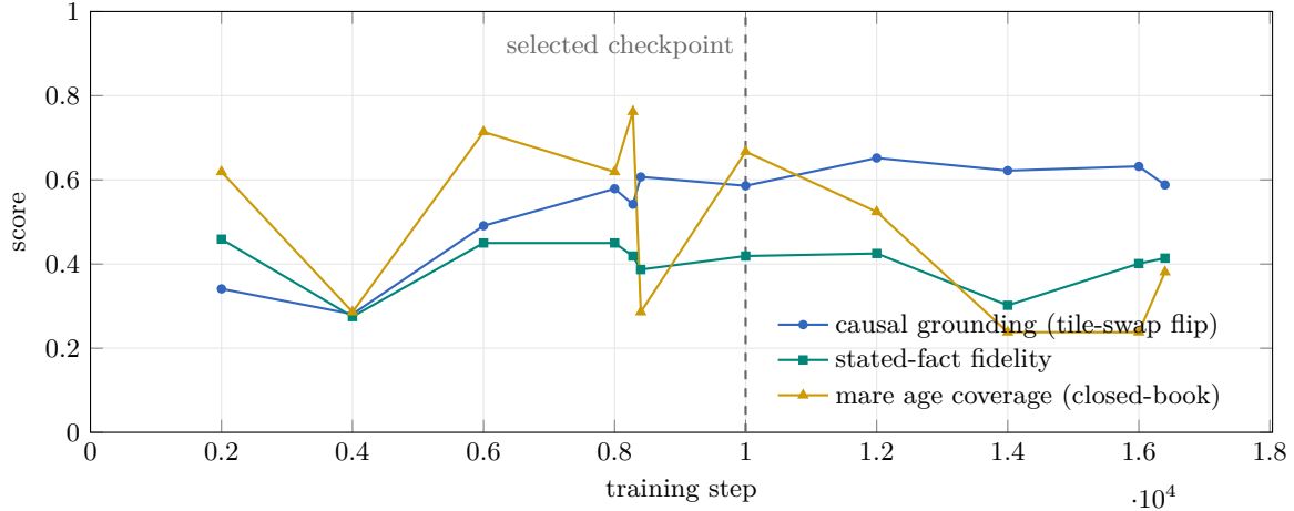
Figure 6: Training dynamics of the bridge. Causal vision grounding (tile-swap flip) trends upward over training, while adherence to target content (stated facts, closed-book age coverage) peaks early and decays. The served checkpoint is selected at the knee of this trade-off, never by validation loss, which measures fit to distilled targets rather than grounding. Late checkpoints additionally degenerate into repetition (not shown).
