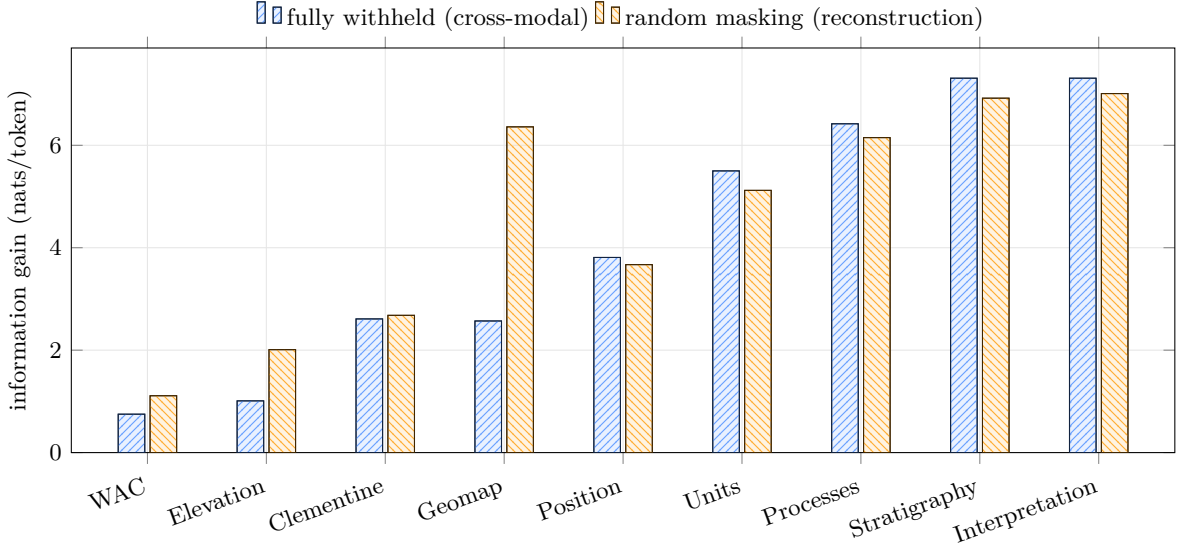
Figure 4: Per-modality predictability in one comparable unit, computed as the uniform-vocabulary NLL floor minus the measured token NLL (nats per token), with the target modality fully withheld (cross-modal) or partially masked as in training (reconstruction). Structured modalities (captions, geologic map) are largely recoverable from the co-registered context. Raster token identity is not, although decoded rasters remain perceptually faithful (Table 2).
