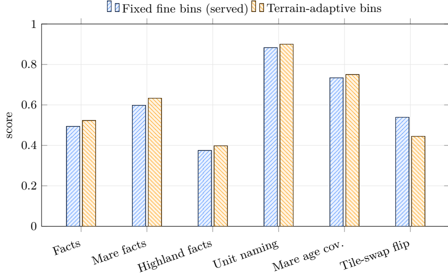
Figure 7: Terrain-adaptive bins vs. the served fixed fine bins on the identical seeded held-out tiles (Table 5). Adaptive bins win every content metric, highland fact fidelity most of all, but lose causal grounding (paired tile-swap \Delta = -0.093 , t = -3.90 ), the axis on which the serving decision is gated.
