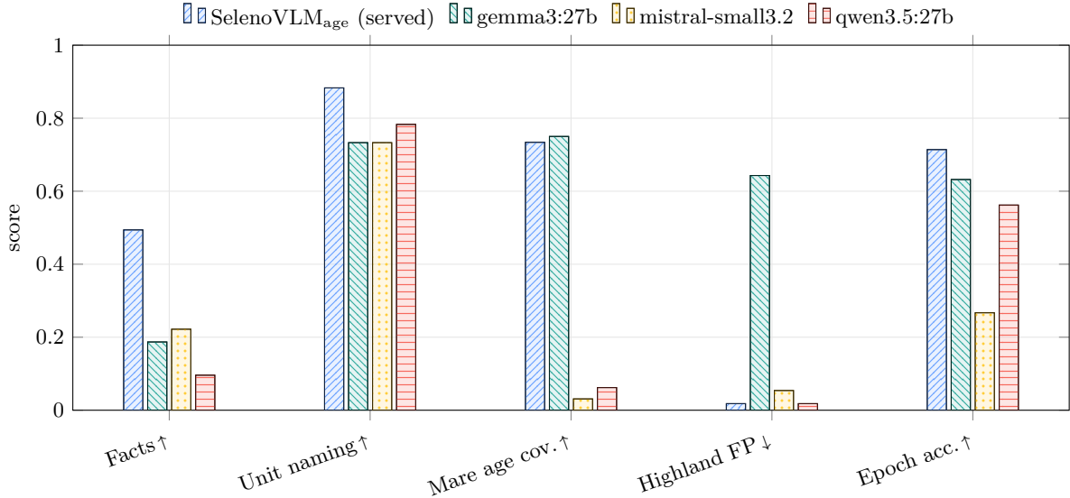
Figure 5: Instructed open (V)LM baselines vs. SelenoVLM age on identical tiles, protocol, and scoring. The baselines are fluent and image-reactive but read quantities poorly, and none combines mare age coverage with highland silence. Arrows on the category labels mark whether a higher ( \uparrow ) or lower ( \downarrow ) score is better, the highland false-positive rate being the only category where lower is better.
